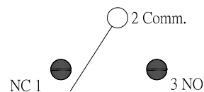
P.C.B MOUNTING
