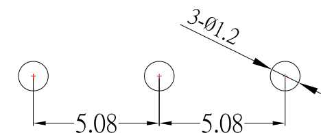
P.C.B LAYOUT MOUNTING
