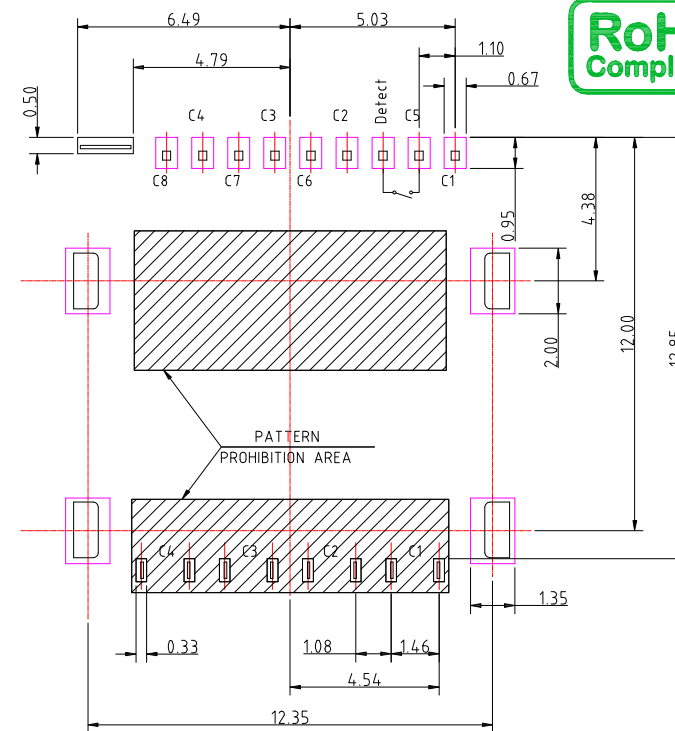
PCB LAYOYT
