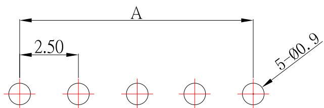
P.C.B LAYOUT MOUNTING PATTERN
