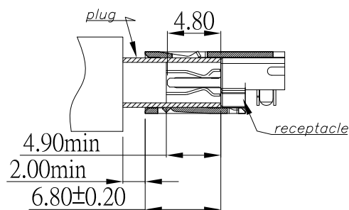
Mated Condition
