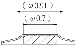
Actuator cross section (Section C-C)
