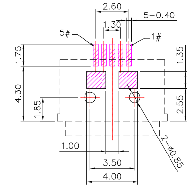
P.C.B LAYOUT MOUNTING PATTERN TOP VIEW
