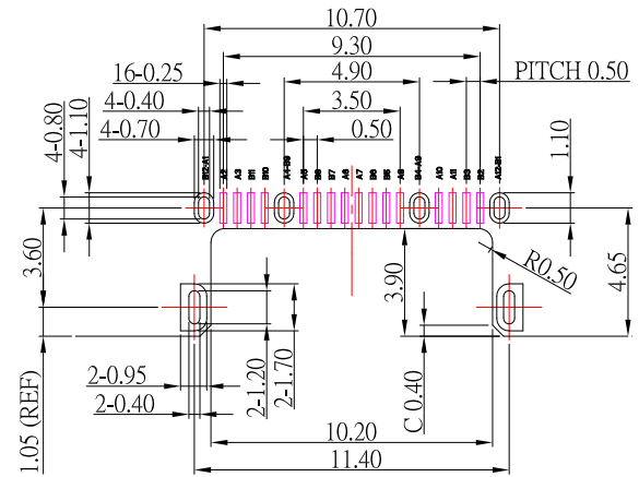
RECOMMEND P.C.B LAYOUT (COMPONENT SIDE)
