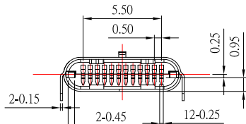
P.C.B LAYOUT MOUNTING PATTERN
