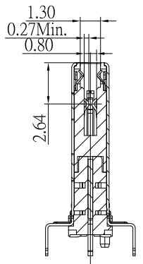
SECTION: B-B
