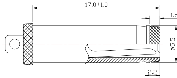
RECOMMENDED PLUG
