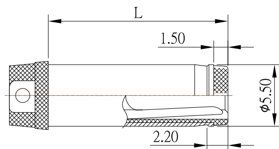
RECOMMENDED PLUG
