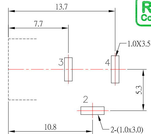
P.C.B LAYOUT MOUNTING PATTERN (TOP-VIEW)
