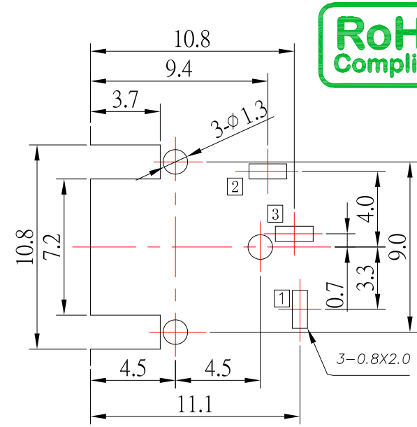
PCB LAYOUT
