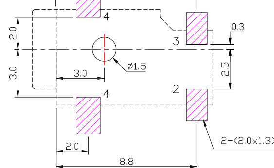
P.C.B LAYOUT MOUNTING PATTERN (TOP VIEW)
