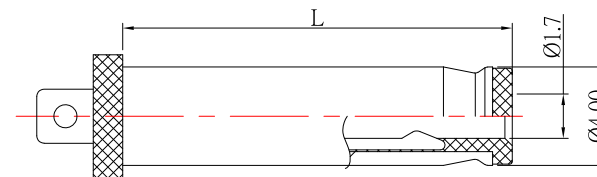
RECOMMENDED PLUG
