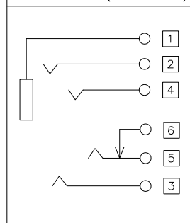
SCHEMATIC(PLUG OUT)
