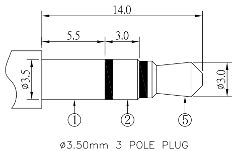
3.50mm 3 POLE PLUG
