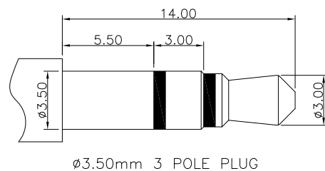
Ø3.50mm 3 POLE PLUG
