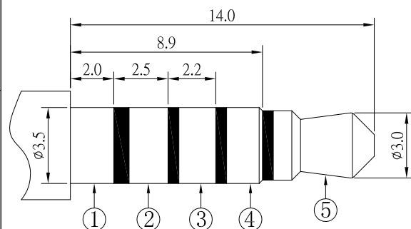
ø3.50mm 5 POLE PLUG
