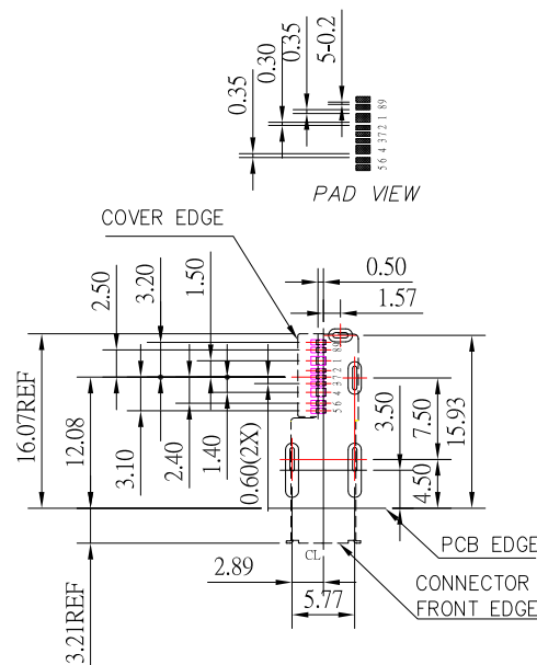
Recommend PCB Layout Top View
