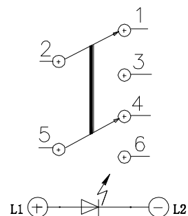
CIRCUIT DIAGRAM
