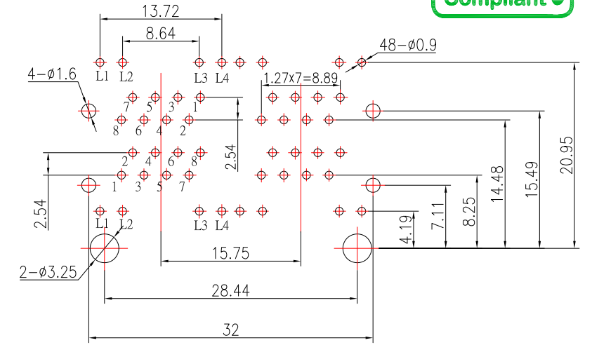
PCB LAYOUT
