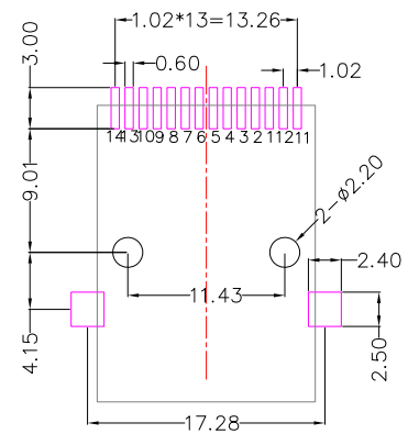
PCB LAYOUT
