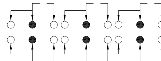
SCHEMATIC (NON-SHORTING)
