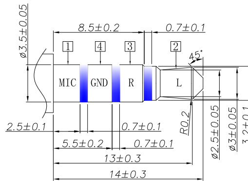
Matching Plug
