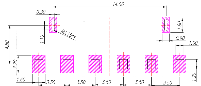
PCB LAYOUT
