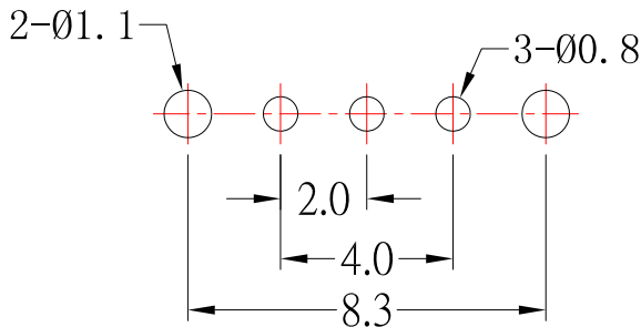
P.C.B MOUNTING PATTERN
