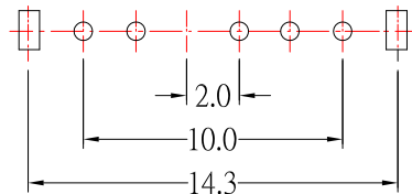
P.C.B MOUNTING PATTERN
