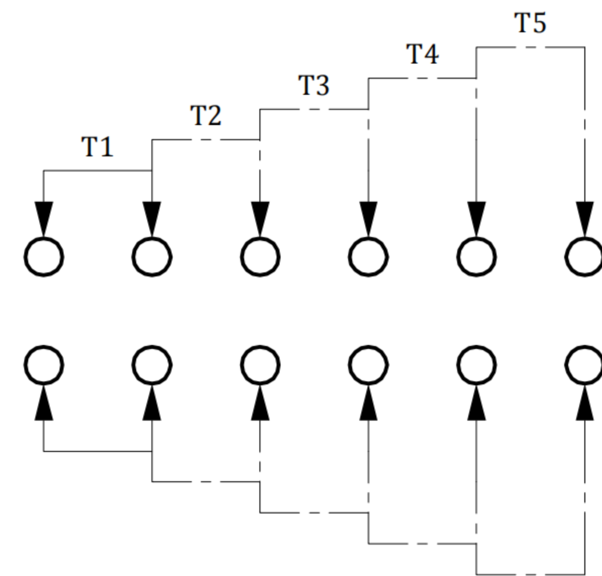
SCHEMATIC(SHORTING)
