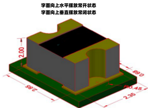
AS-X24-45-1210-L2.85xW2.35xH2.0mm
